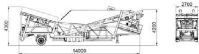
TRANSPORT POSITION
